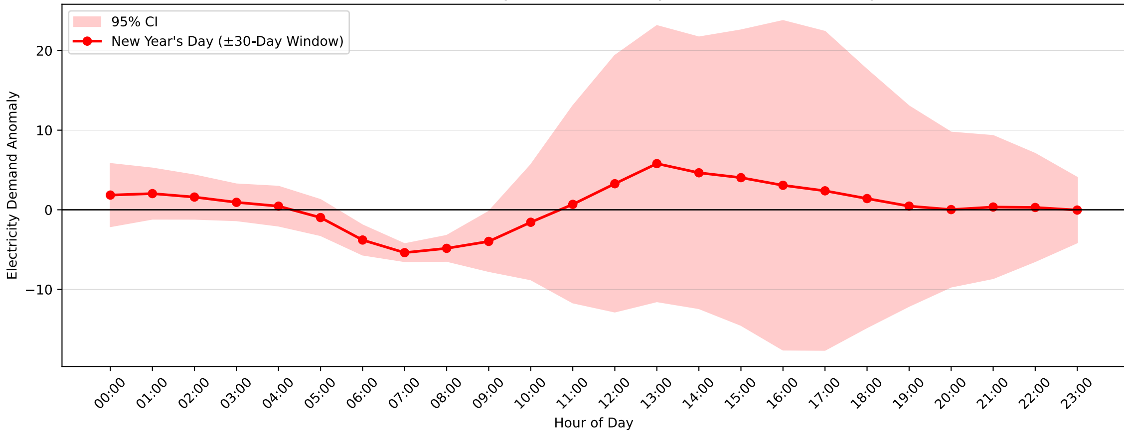
Pennant Hills Demand Anomaly: New Year's Day (2013–2014, \pm 30 -Day Window)
