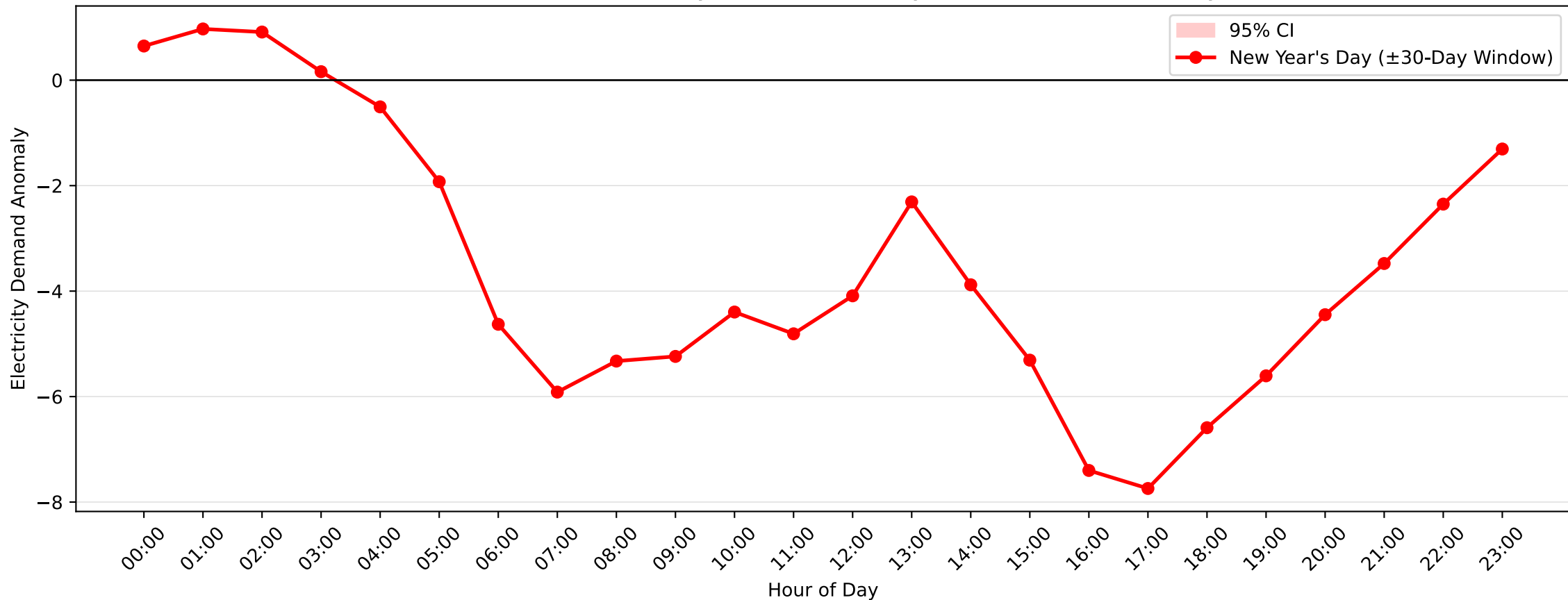
Pennant Hills Demand Anomaly: New Year's Day (2014-2015, \pm 30 -Day Window)
