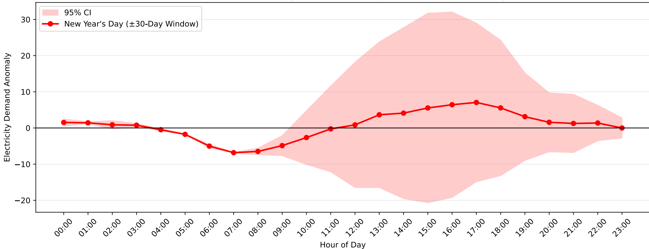
Pennant Hills Demand Anomaly: New Year's Day (2010-2011, \pm 30 -Day Window)
