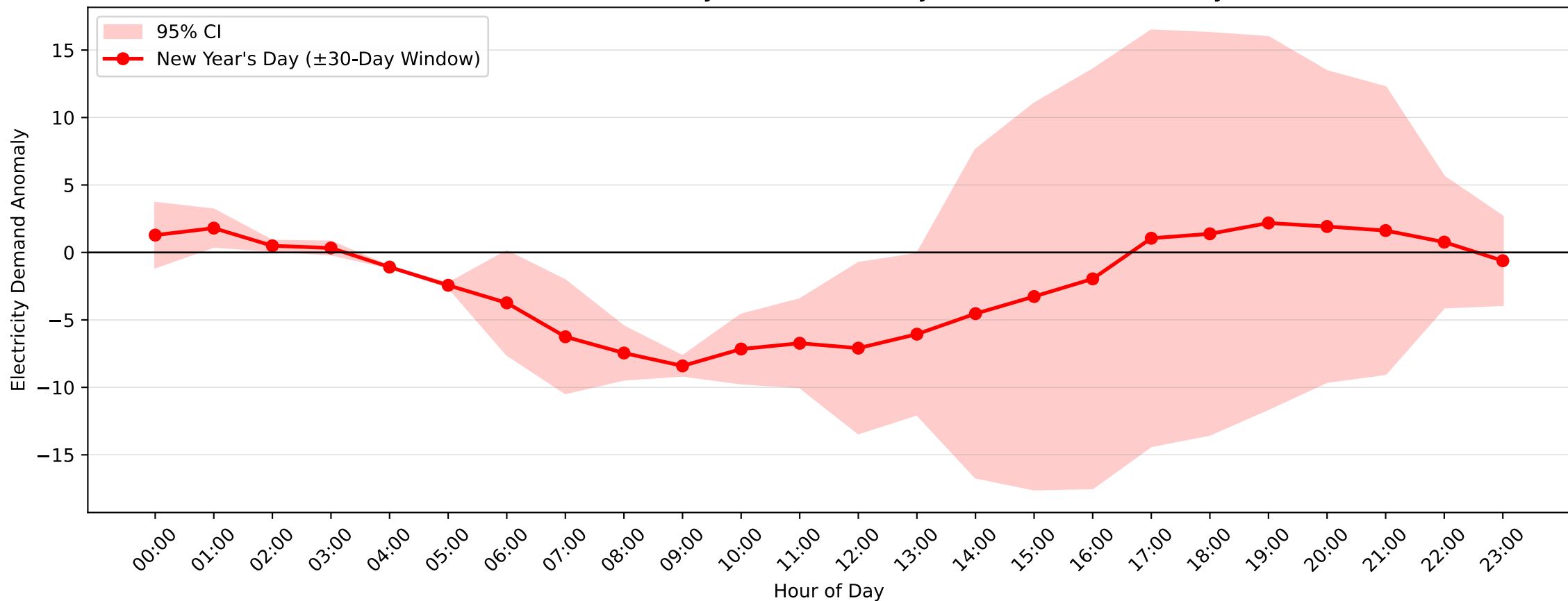
Pennant Hills Demand Anomaly: New Year's Day (2009–2010, \pm 30 -Day Window)
