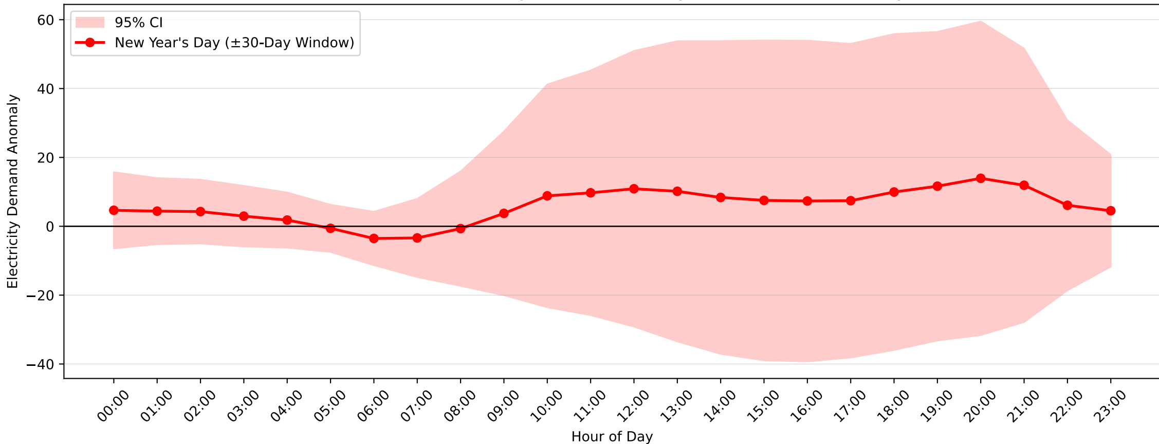
Pennant Hills Demand Anomaly: New Year's Day (2006–2007, \pm 30 -Day Window)
