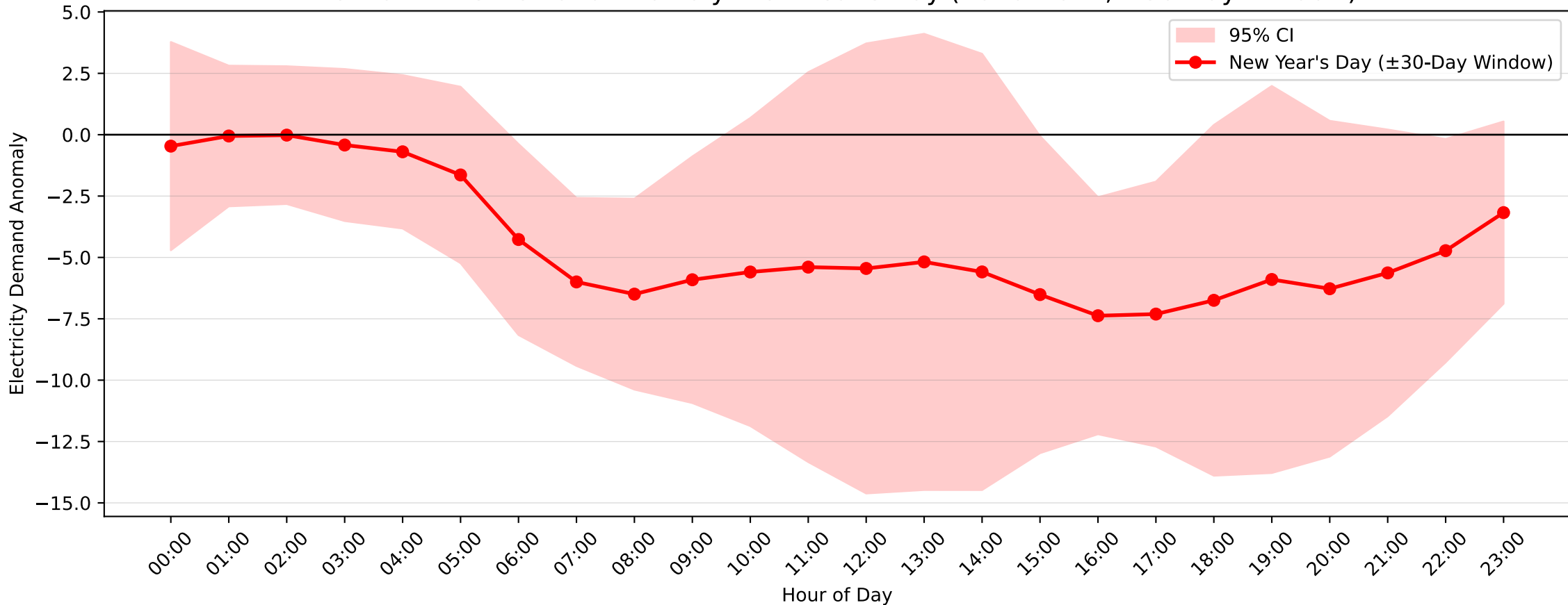
Pennant Hills Demand Anomaly: New Year's Day (2016-2017, \pm 30 -Day Window)
