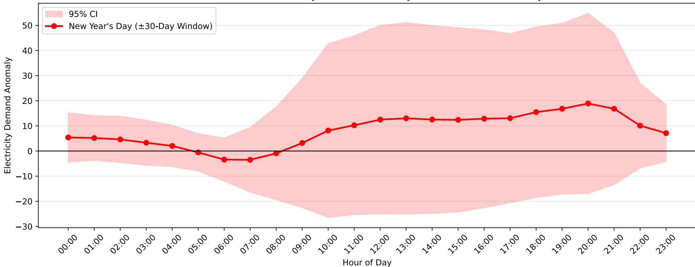
Pennant Hills Demand Anomaly: New Year's Day (2005–2006, \pm 30 -Day Window)
